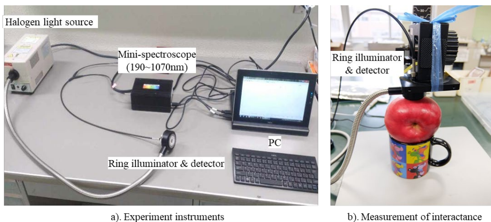
Figure 2. Instruments and experimental setup.
