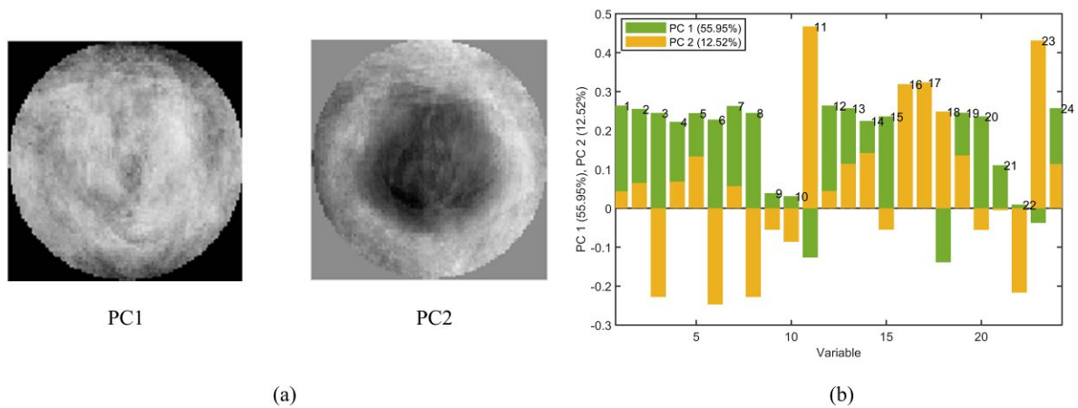
Figure 4. Loadings of principal component analysis; (a) full pixel (b) color features (where 1, 2, and 3 means mean of RGB. 4, 5, and 6 means mean of normalized RGB. 7, 8, and 9 means mean of YCbCr. 10, 11, and 12 means mean of HSV. 13, 14, and 15 means standard deviation of RGB. 16, 17, and 18 means standard deviation of normalized RGB. 19, 20, and 21 means standard deviation of YCbCr. 22, 23, and 24 means standard deviation of HSV.)
