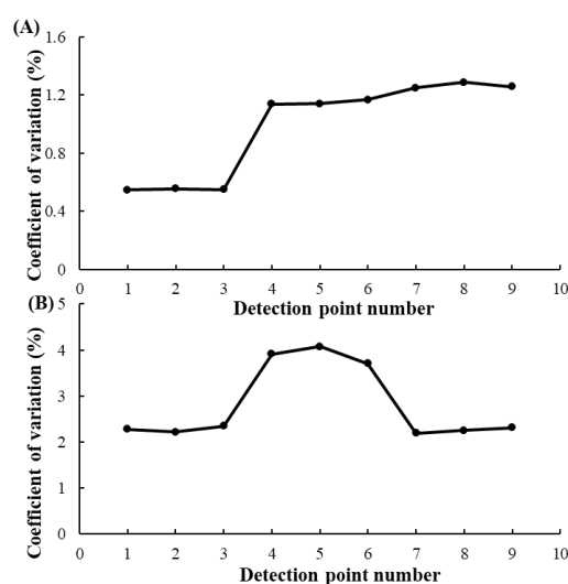
Figure 12. The coefficient of variation of resonant frequency (A), the peak value (B) in different detection points.
