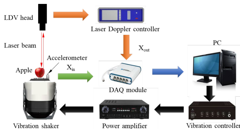
Figure 2. A vibration generator-based LDV detection system.
