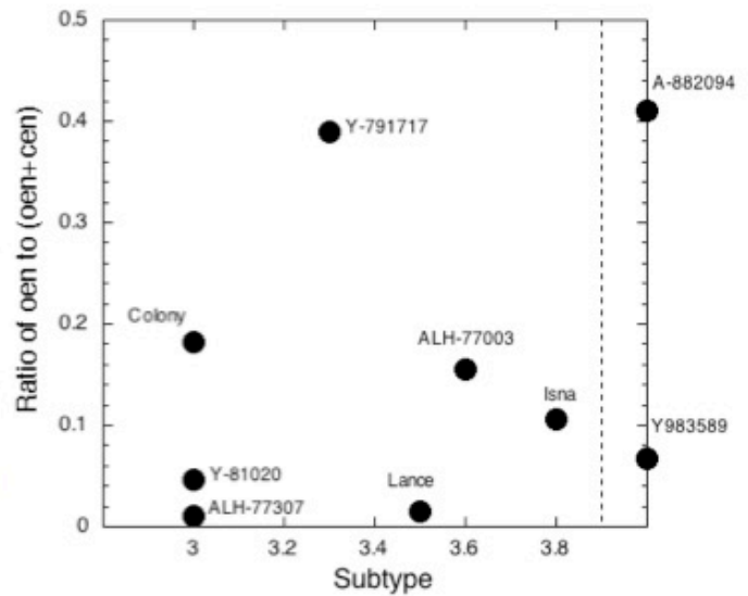
Fig. 2. The ratios of orthoenstatite (oen) to two phases of enstatites (opx+cpx) for various subtypes of the CO3 chondrites. Cen=clinoenstatite.
