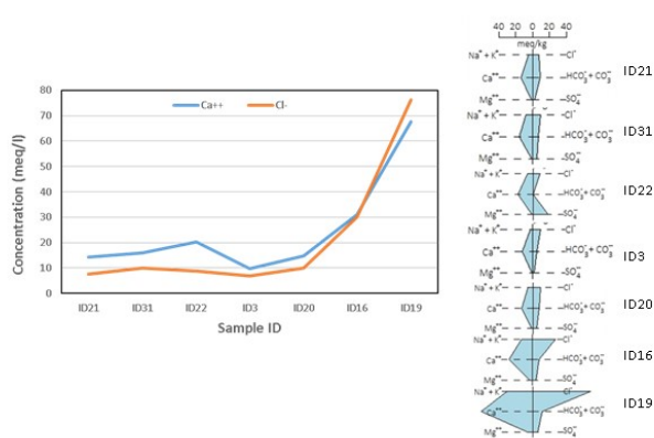
Fig 3. \text{Ca}^{++} and \text{Cl}^- pattern along Cimanuk River (Rusydi, 2017)
