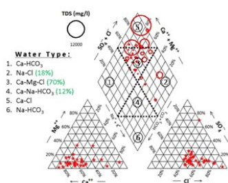
Fig 2. Piper diagram
