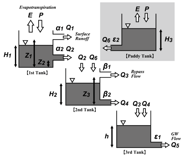
[Tank model structure]
