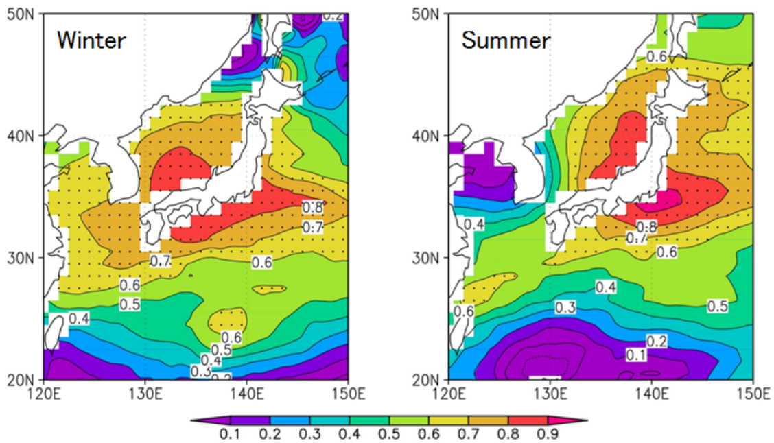
Fig. 1 Correlation coefficients between SAT over Japan and SST around Japan in winter (left) and summer (right). Both SAT and SST data are detrended and filtered with 5-year running mean. Stippling indicates the area where correlation coefficients are statistically significant at the 95% confidence level.
