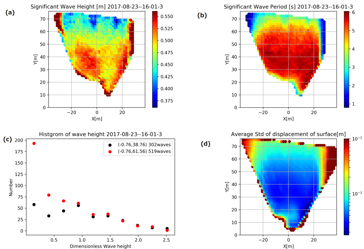
Figure. Spatial distribution of significant wave height (a) and period (b) when the value of them from ultra-sonic wave gauge were 0.513 m and 6.1 s. X axis in the figure is parallel to baseline of stereo camera.
