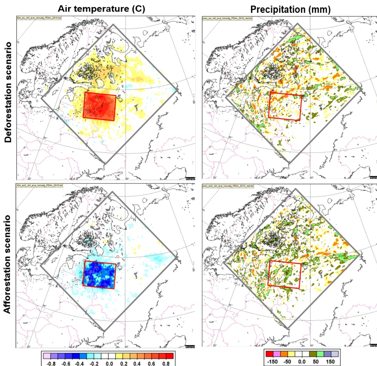
Figure 1. Simulated differences in the air temperature (°C) and precipitation rate (mm) for the selected model domain between the deforestation and afforestation scenarios of the model region and the control experiment, assuming present land-use structure
