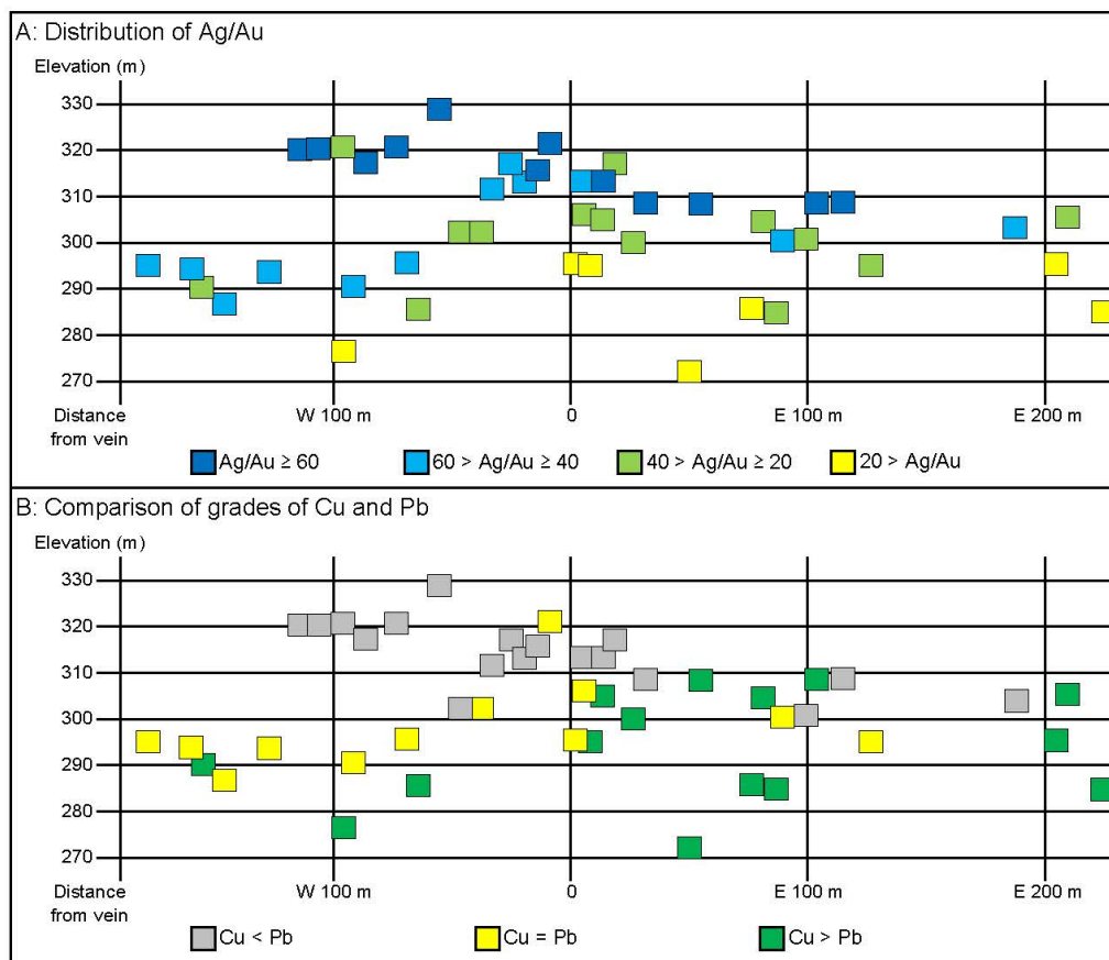
Fig. 1 Ag/Au value, and grades of Cu and Pb in the type-I mineralization, plotted on the longitudinal section of the vein.
