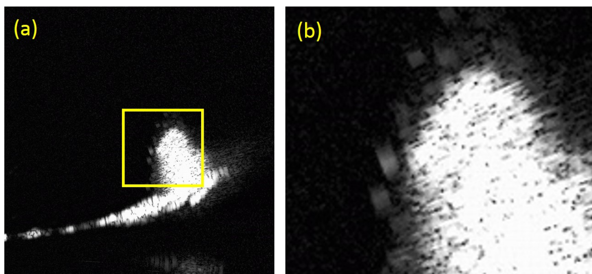
Fig. 1 Volcanic eruption column 2 minute after eruption observed by X-band marine radar. 22:11 LST, May 4, 2018.
