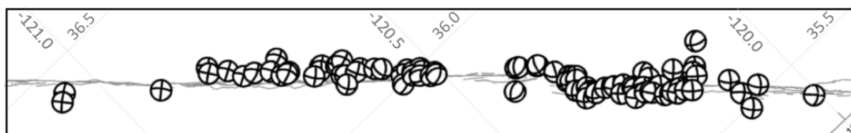
Figure 1 . The focal mechanisms of LFE families
