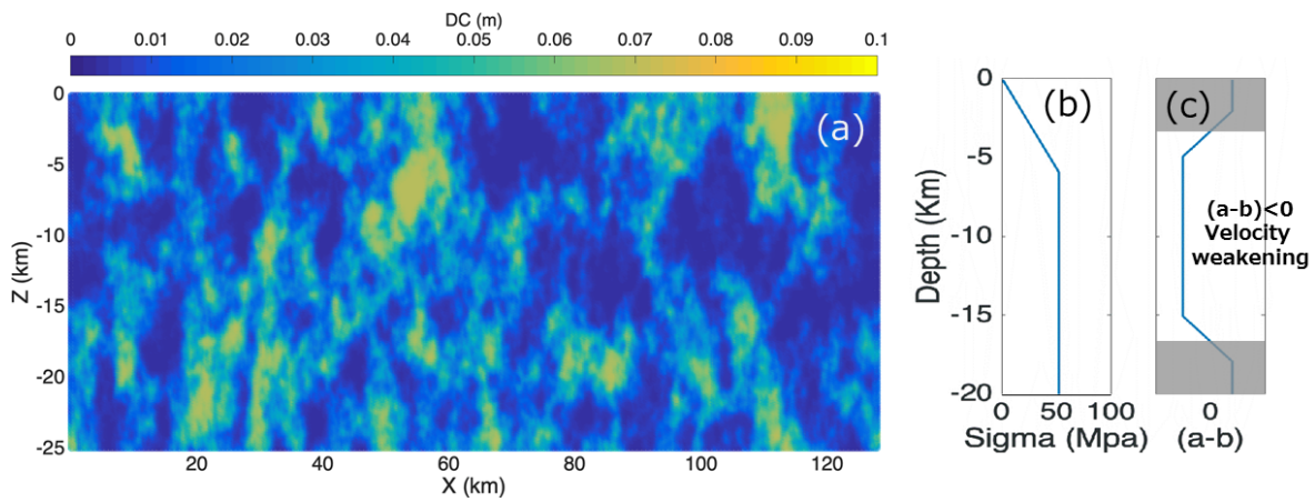
Fig 1. Friction settings: (a) heterogeneous D_c , (b) normal stress, and (c) a-b friction parameters.
