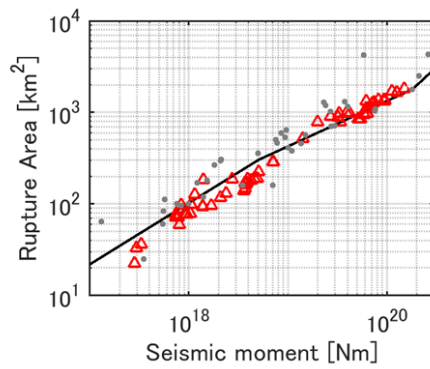
Fig 2. Comparison of S -values of modeled events vs. M_0 (triangles) and observed (dots). Line is 3-stage scaling assumed for strong-motion simulations.
