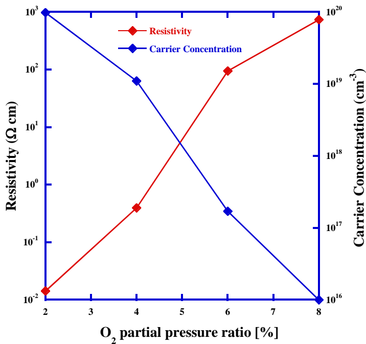
Fig. 2 Resistivity and Carrier Concentration of GZO
