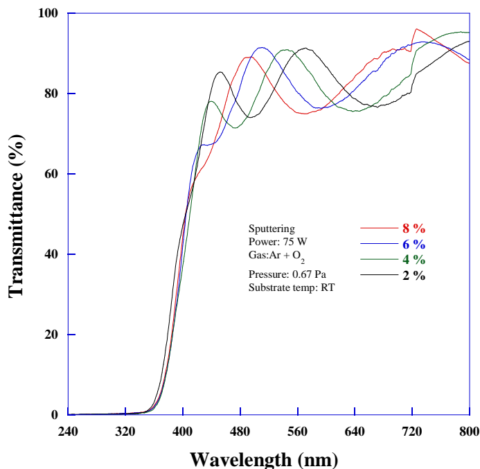
Fig. 1 Transmittance of O 2 pressure ratio of GZO
