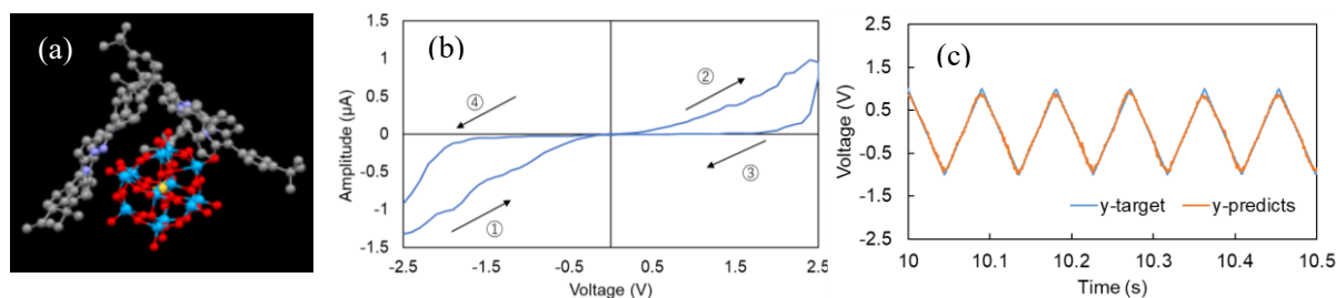
Fig.1 (a): POM(SV 2 W 10 O 40 /H 4 t-BuTPP) molecular structure. (b): I-V curve of random network device. The sweep order was indicated by arrows in numerical order. (c): Result of waveform generation task. Predicts wave form made by linear combination of several output signals from the device were following to a target signal. MSE is mean square error.
