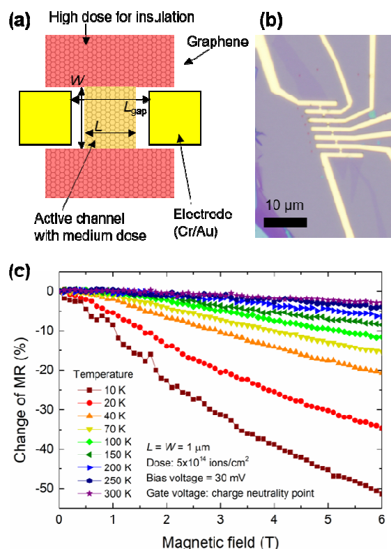
Fig. 1. (a) Schematic design of helium-ion-irradiated graphene device in this work. (b) Optical image of the typical device. (c) MR as a function of magnetic field for various temperatures.
