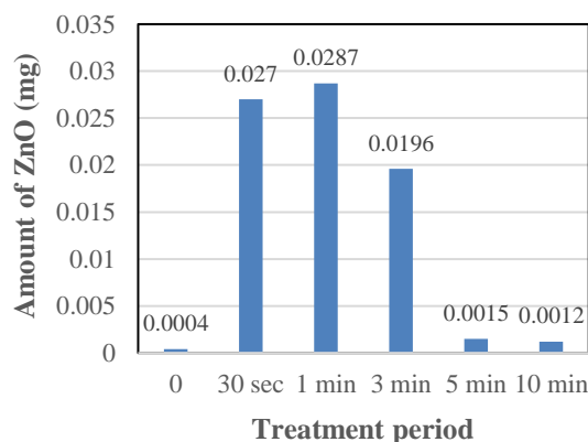
Fig. 2 Production amount of ZnO in water varying the ozone treatment period.
