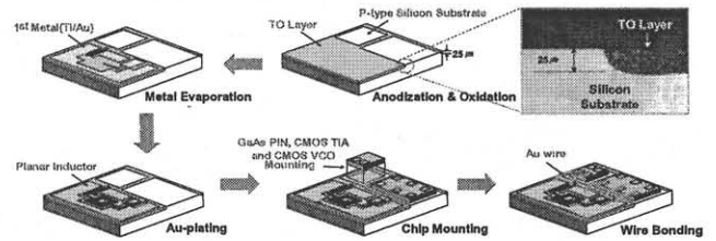
Fig. 7 Fabrication process of MCO and Thick Oxide
