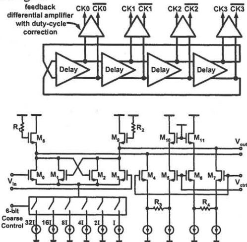
Fig. 2 4-stage VCO with an active inductor loaded delay
