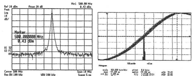
Fig. 3 Spectrum and jitter histogram of the recovered clock
