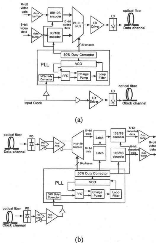
Fig. 4 Block Diagrams of the 5-channel CMOS (a) transmitter and (b) receiver
