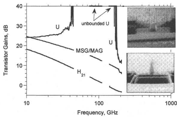
Fig. 1 : Measured mm-wave gains of an InAlAs / InGaAs / InGaAs deep submicron transferred-substrate HBT.
