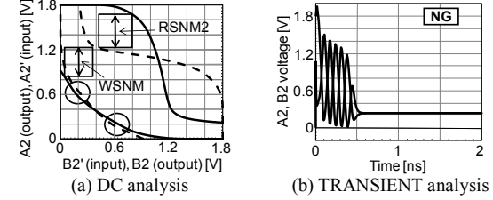
Fig. 7. Correlation between SNM (DC) and oscillation (TRANSIENT)
