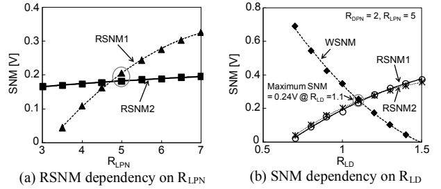
Fig. 8. Optimization of the oscillator circuit.
