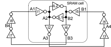
Fig. 2 The oscillator circuit re-drawn like an SRAM cell.
