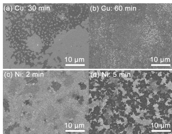
Fig. 1: SEM images of graphene with different morphologies grown on (a, b) Cu and (c, d) Ni substrates.
