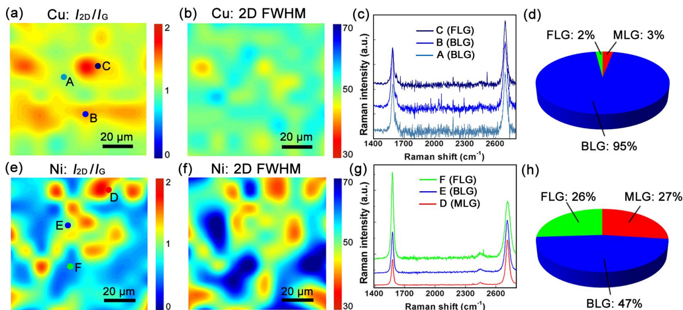
Fig. 2: Raman spectroscopic analyses of as grown graphene after transferred on Si/SiO 2 substrates. Raman maps of I_{2D}/I_G and 2D FWHM of graphene grown on (a, b) Cu and (e, f) Ni. (c, g) Raman spectra of three corresponding points in (a, e). The percentages of MLG, BLG and FLG graphene grown on (d) Cu and (h) Ni.
