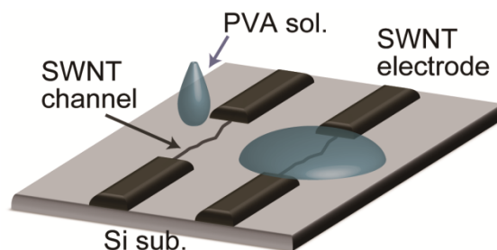
Fig. 1 Schematic of CNT-FET device structure.
