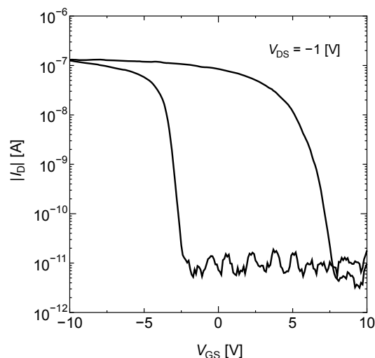
Fig. 2 Typical transfer characteristics of as-fabricated CNT-FET.
