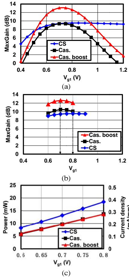
Fig. 3 (a) Simulated maximum gain with different bias voltages, (b) measured maximum gain with different bias voltages, (c) measured power consumption and current density.
