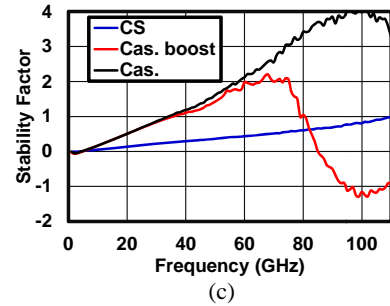
Fig. 2 The measured maximum gain, S_{12} and stability factor of the CS, cascode, and gain-boost cascode topologies, (a) maximum gain, (b) S_{12} , (c) stability factor.
