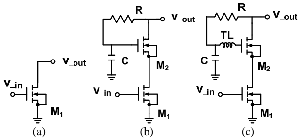
Fig. 1 (a) CS topology, (b) cascode topology, (c) Gain-boost cascode topology.
