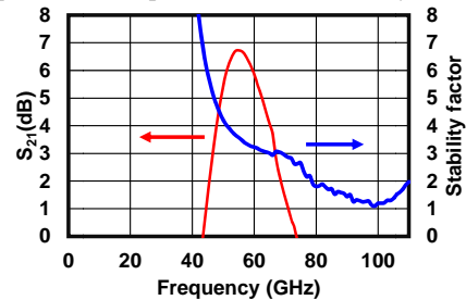
Fig. 4 Measure power gain and stability factor of one-stage amplifier.
